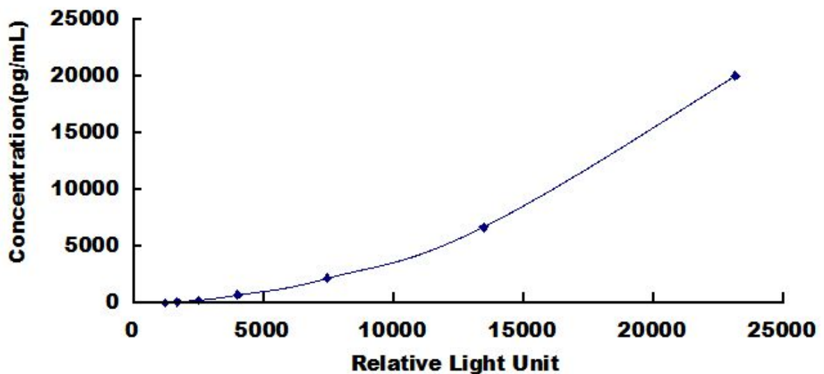
Typical Standard Curve for MMP3, Rat CLIA.
